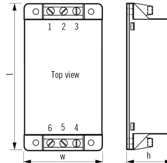
Chassis mounting with Screw Terminal Block
