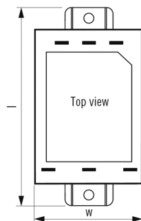
Chassis mounting with Faston-Tabs
